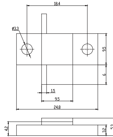
UCL-HPR50GB
