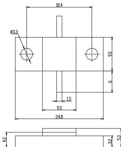
UCL-HPR100A
