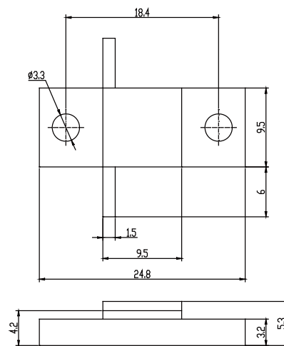
UCL-HPR100B
