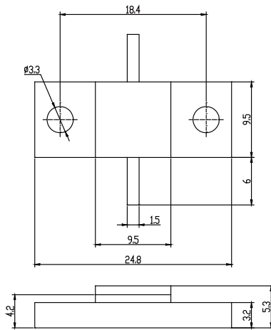
UCL-HPR50GA
